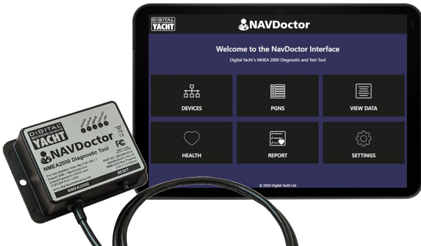
Digital Yacht's Diagnosetool NAVDoctor
